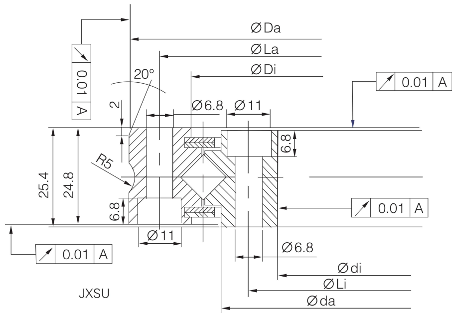
Integral outer and inner ring with mounting holes
